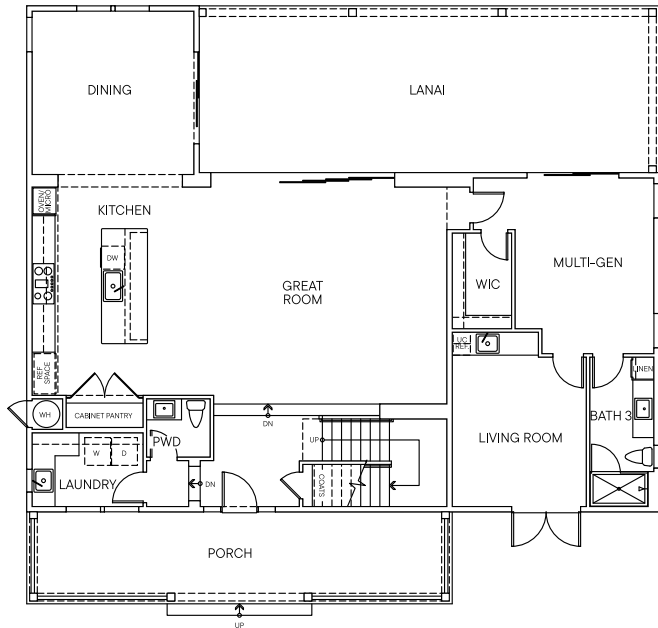
FIRST FLOOR (SHOWN W/ OPTIONAL MULTI-GEN SUITE)
